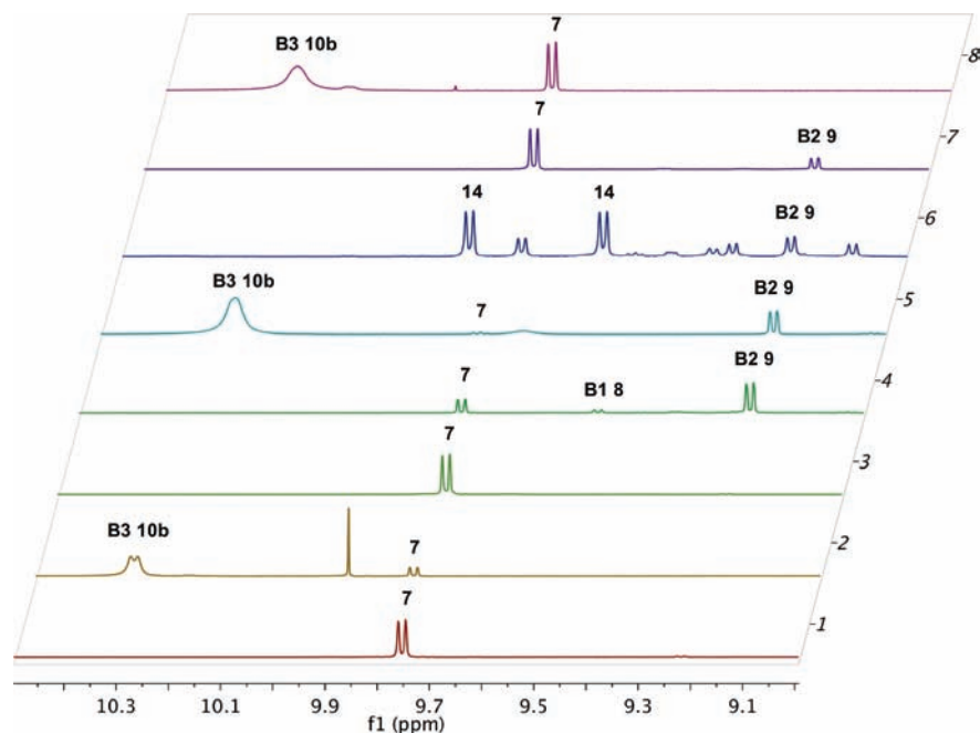
Figure 1. ^1\text{H} NMR spectra of the reaction mixture (Scheme 2) in \text{CDCl}_3 with \text{Ph}_3\text{CH} as internal standard. Entry 1: ( S )-VAPOL plus 3 equiv \text{B(OPh)}_3 at 25 °C for 10 min. Entry 2: ( S )-VAPOL plus 3 equiv \text{B(OPh)}_3 and 2 equiv imine 1b at 25 °C for 10 min. Entry 3: ( S )-VAPOL plus 3 equiv \text{B(OPh)}_3 and 2 equiv aziridine 3b at 25 °C for 10 min. Entry 4: ( S )-VAPOL plus 3 equiv \text{B(OPh)}_3 were heated at 80 °C in toluene for 1 h followed by removal of volatiles under vacuum for 0.5 h. Entry 5: 2 equiv of imine 1b added to the solution in entry 4 for 10 min at 25 °C. Entry 6: 2.4 equiv of ethyl diazoacetate added to the NMR tube containing the solution in entry 5 and kept for 9 days at 25 °C. Entry 7: ( S )-VAPOL plus 1 equiv triphenoxyboroxine 13 at 25 °C for 10 min. Entry 8: 2 equiv imine 1b added to solution in entry 7 for 10 min at 25 °C.
