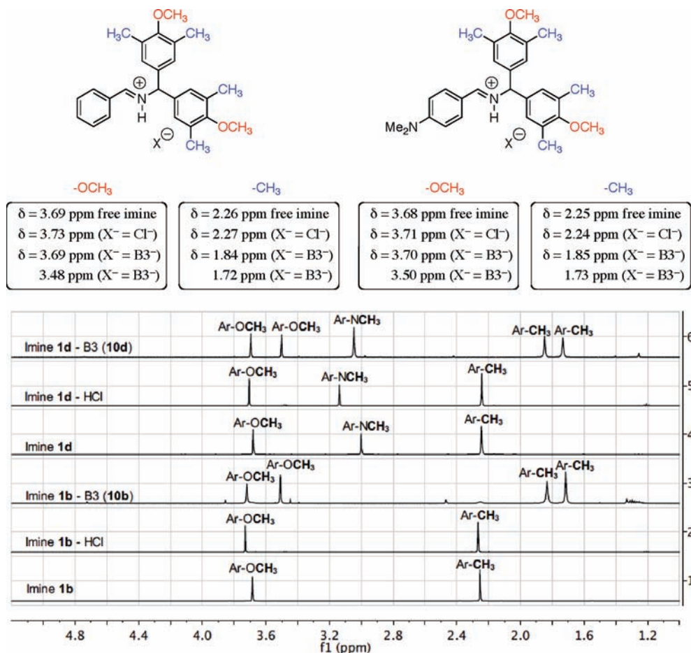
Figure 5. Chemical shifts of methyl and methoxy groups in various imines and iminiums in \text{CDCl}_3 with TMS as internal standard.
